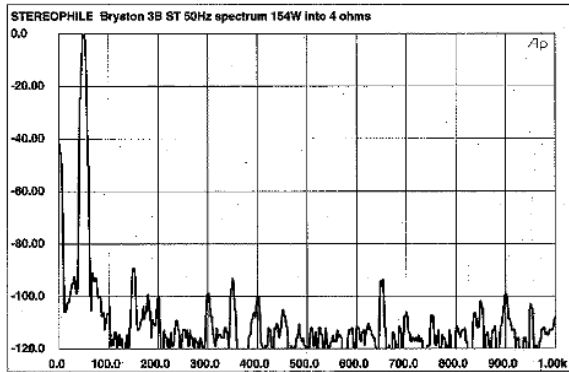
Fig.12 Bryston 3B-ST, spectrum of 50Hz sine wave, DC-1kHz, at 154W into 4 ohms (linear frequency scale).
