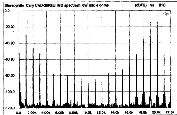
Fig.11 Cary CAD-300SEI, HF intermodulation spectrum, DC-22kHz, 19+20kHz at 6W into 4 ohms (linear frequency scale).
